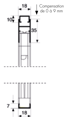
Section Verticale
