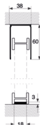
Section Verticale
